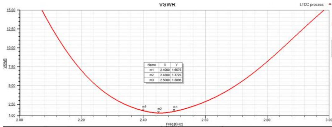
Product Characteristic Curve
